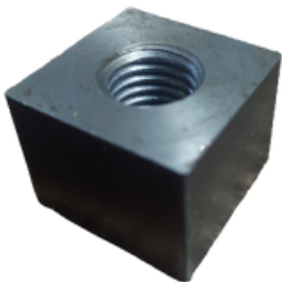
Square 28 x 22 M14
